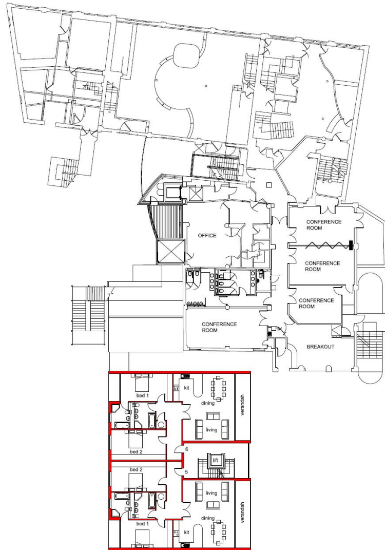
second floor plan 1:200
