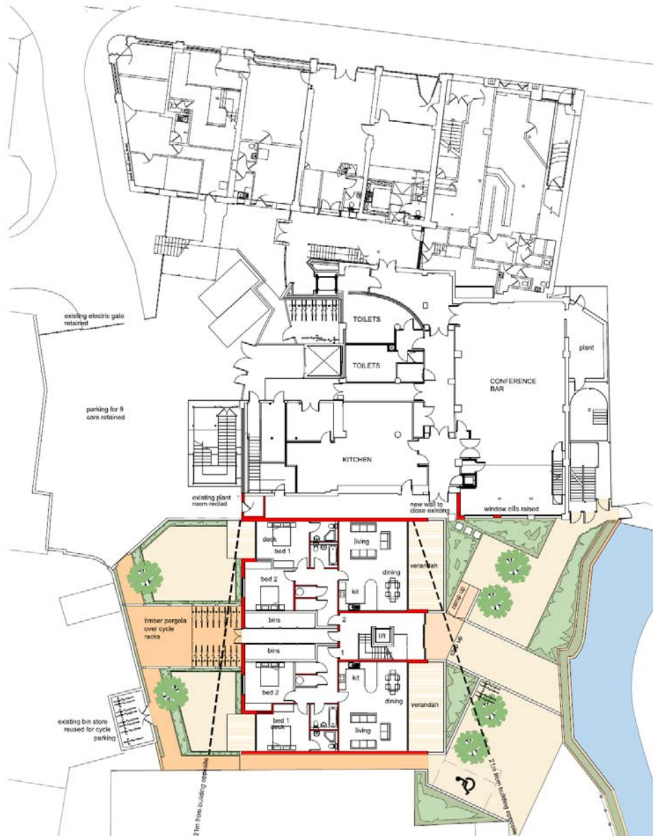
ground floor plan 1:200
